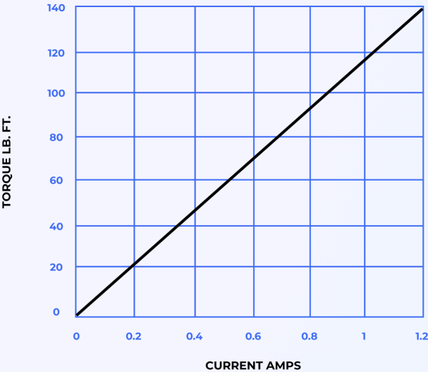
TORQUE VS. COIL CURRENT
