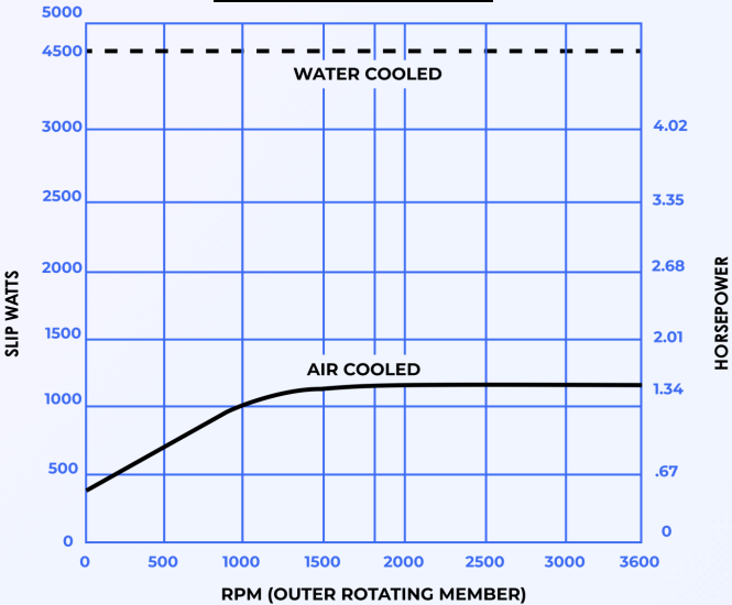
HEAT DISSIPATION VS. SPEED
