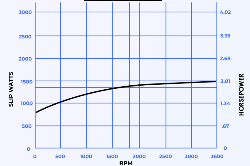
HEAT DISSIPATION VS. SPEED
